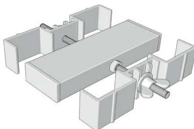
DS-PROSTAGE LEGCLAMP QUAD 1711000042
